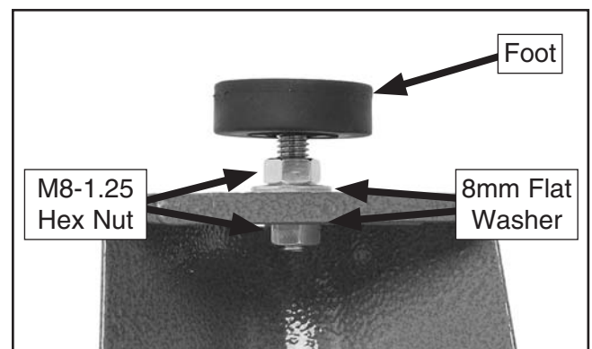
Figure 11. Foot installed with hex nuts and flat washers.
